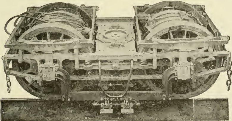
Fig. 256. View of Truck Complete
